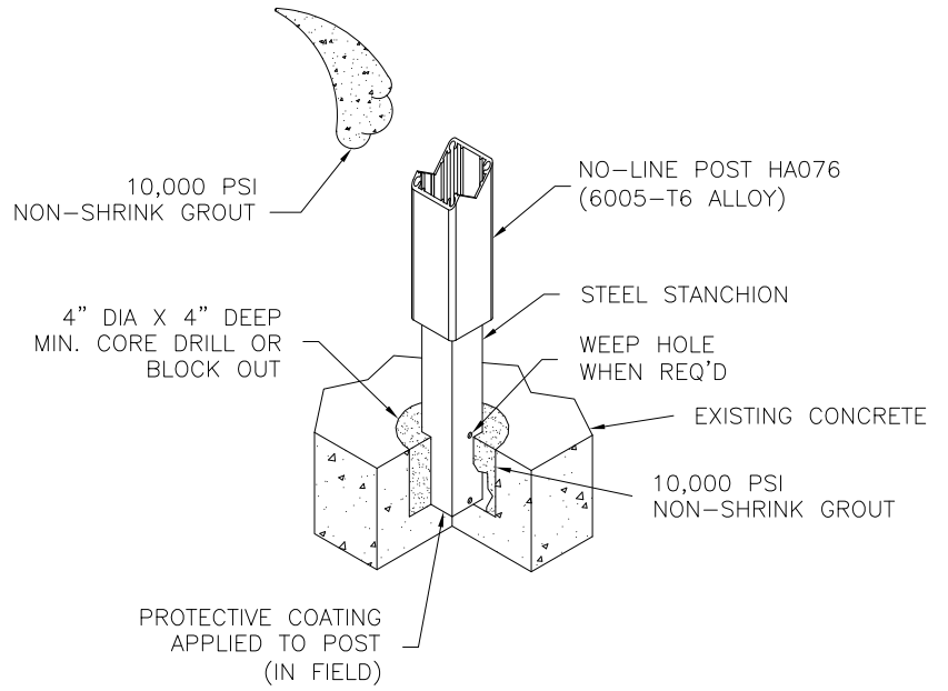
2 STANCHION MOUNTING DETAIL CORE POCKET OPTION SCALE: 3
