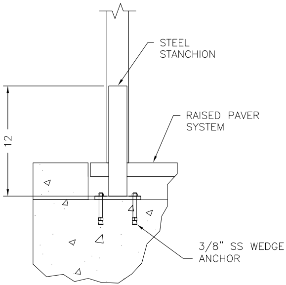
1 STANCHION MOUNTING DETAIL SCALE: 3
