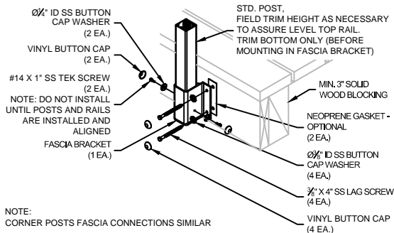
TYP. FASCIA MOUNT TO WOOD CONNECTION
