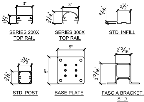
PART PROFILES
