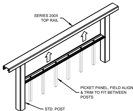
○ TYP. PICKET PANEL TO TOP RAIL CONNECTION
