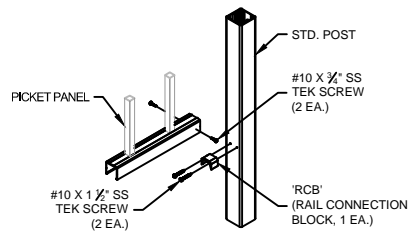
○ TYP. PICKET PANEL TO POST CONNECTION
